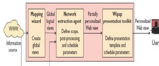
Figure 2. Wiccap system architecture. Each layer in the architecture creates one component of a personalized Web view.
